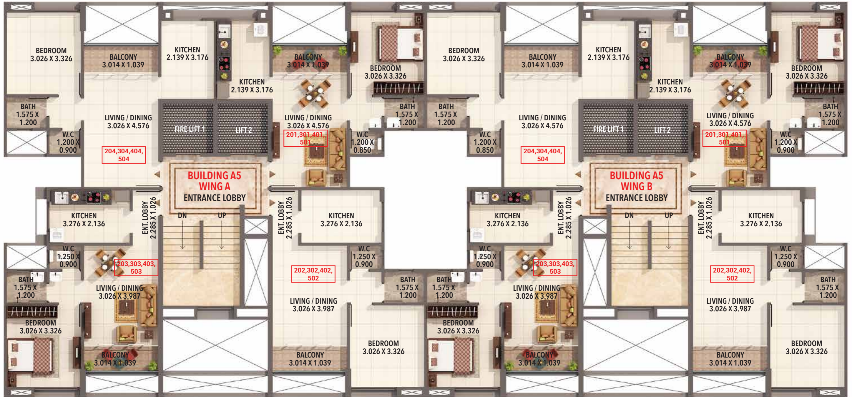
BUILDING A5 - WING A & B (AREAS IN SQ.M)
